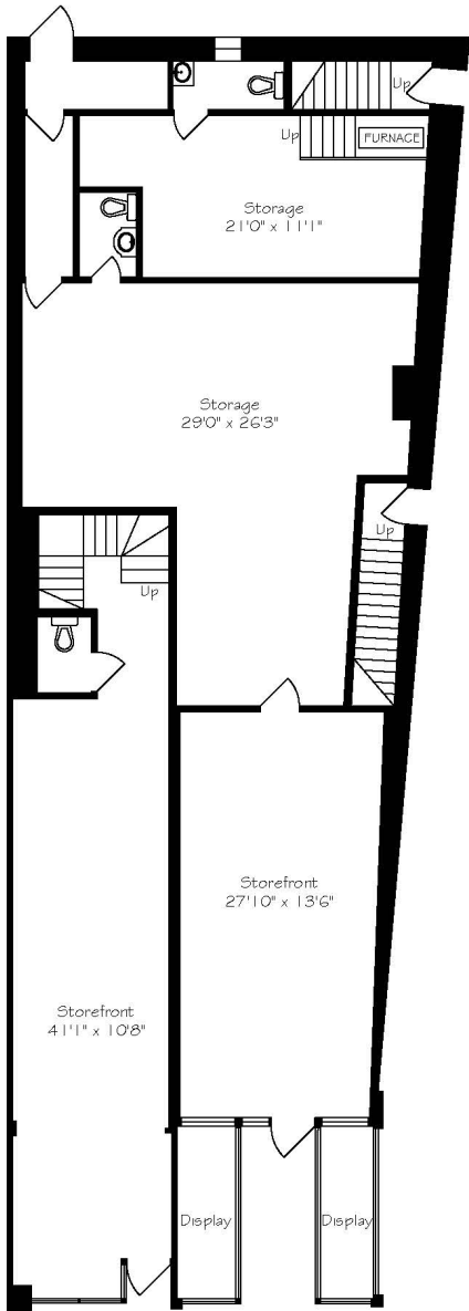
Main Floor Retail
